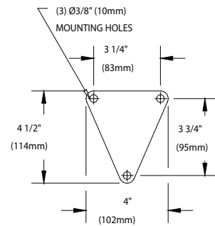
DETAIL "A" MOUNTING BRACKET
